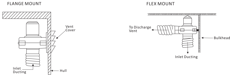
(1) SFBB1-130-01、SFBB2-130-01 DIMENSION.
